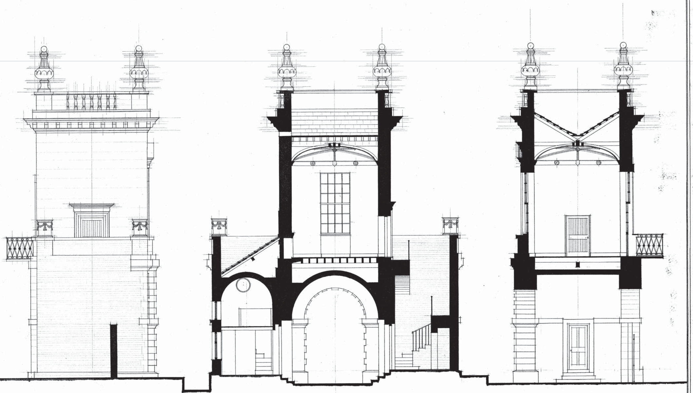
CROSS SECTION
