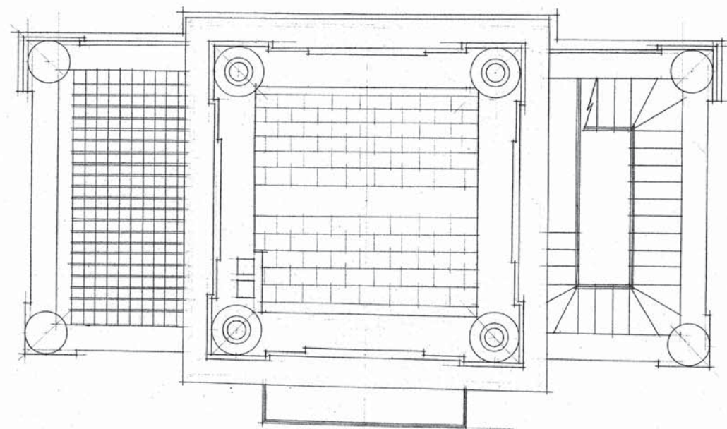
ROOF PLAN.
